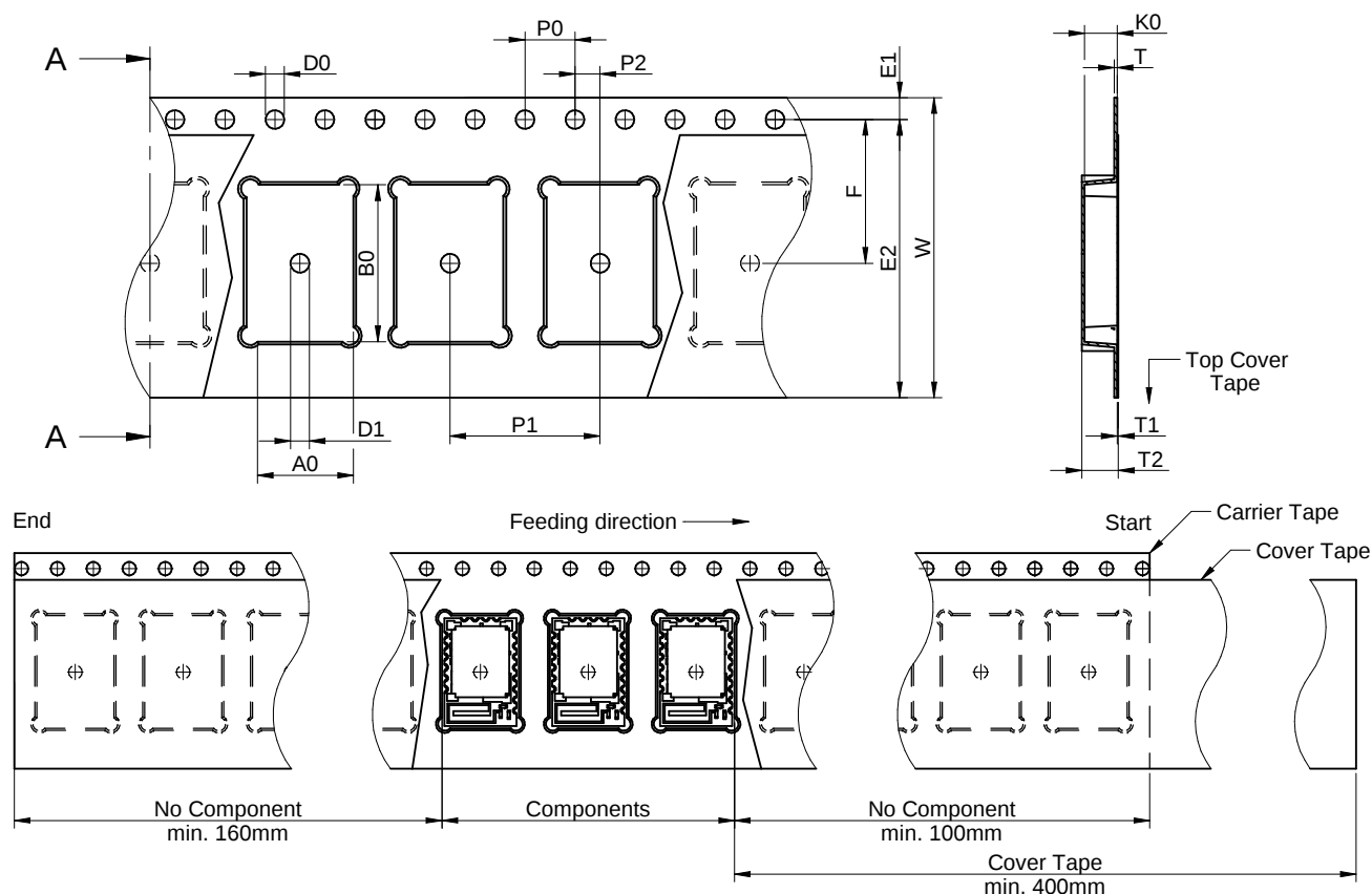
Figure 18: 24 mm Tape
